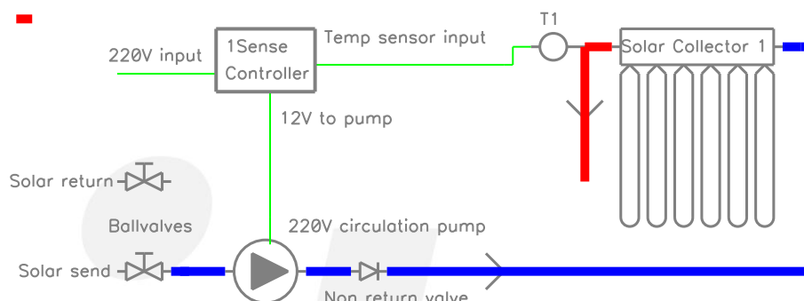
Figure 1: 220V CtrlLite OneSense wiring.
